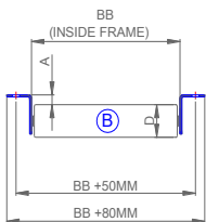
ROLLERS BELOW FRAME B
