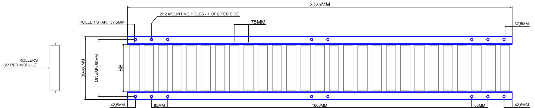
ROLLERS BELOW FRAME
