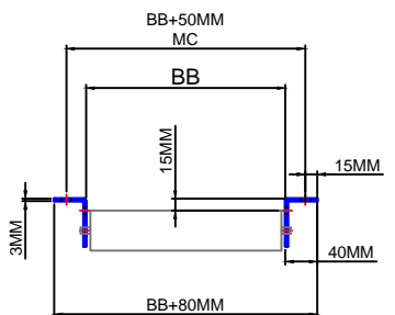
ROLLERS BELOW FRAME
